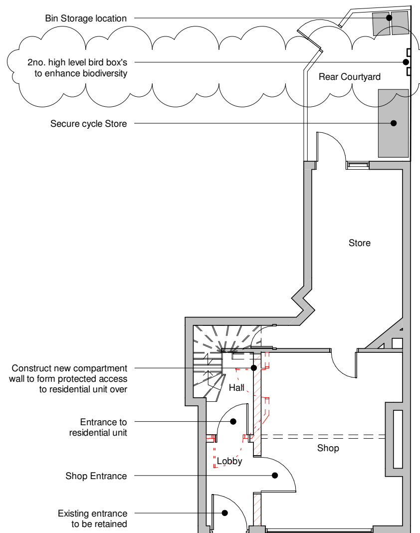
Ground Floor Plan as Proposed 1 : 100
