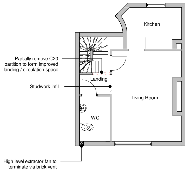
First Floor Plan as Proposed 1 : 100
