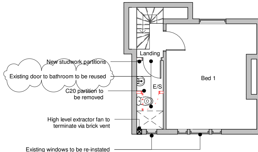
Second Floor Plan as Proposed 1 : 100
