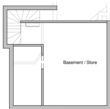
Basement Plan as Proposed 1 : 100
