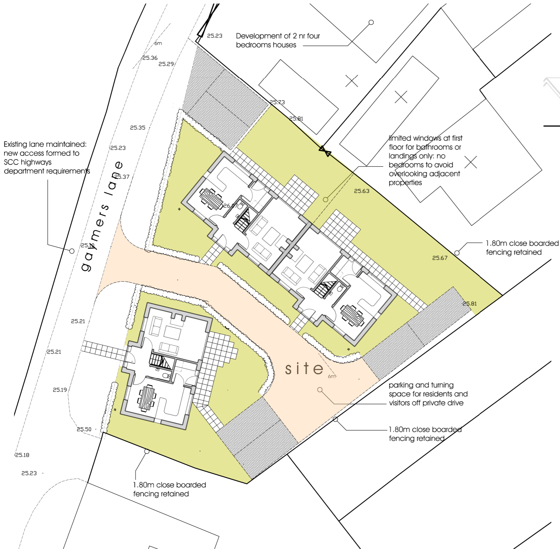
indicative site layout 1:200
