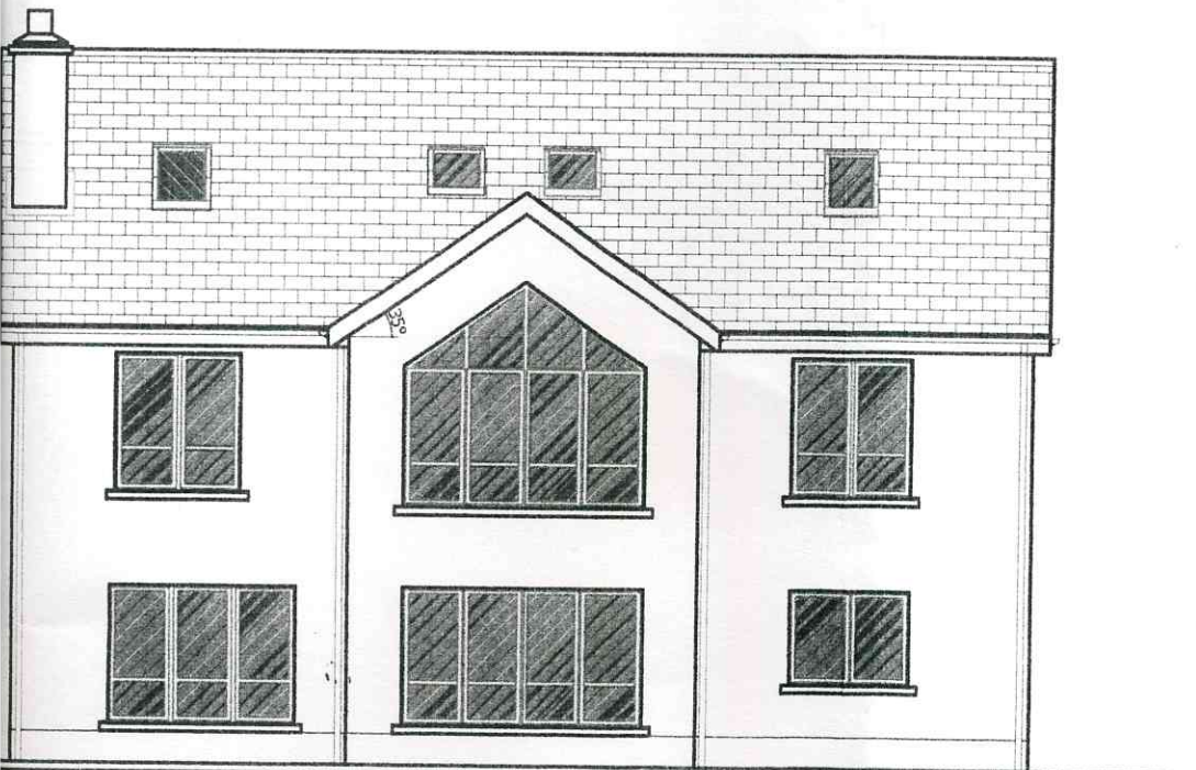
WEST ELEVATION
