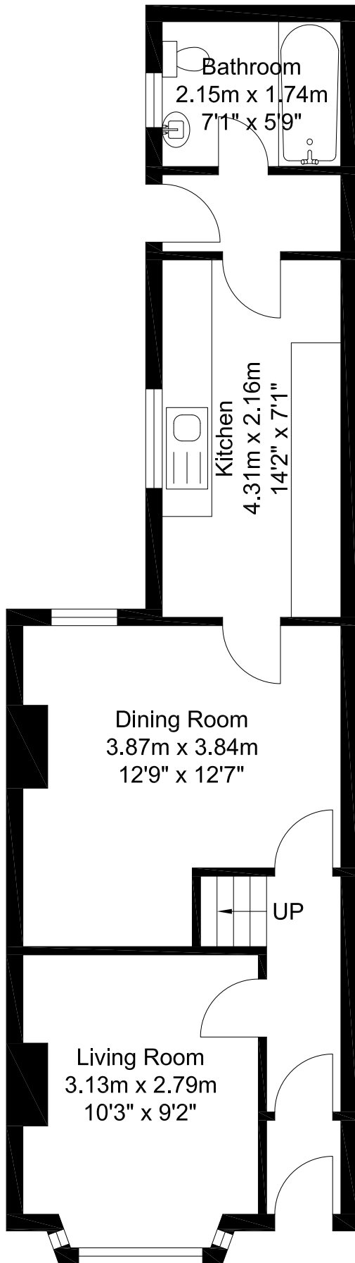
Ground Floor
