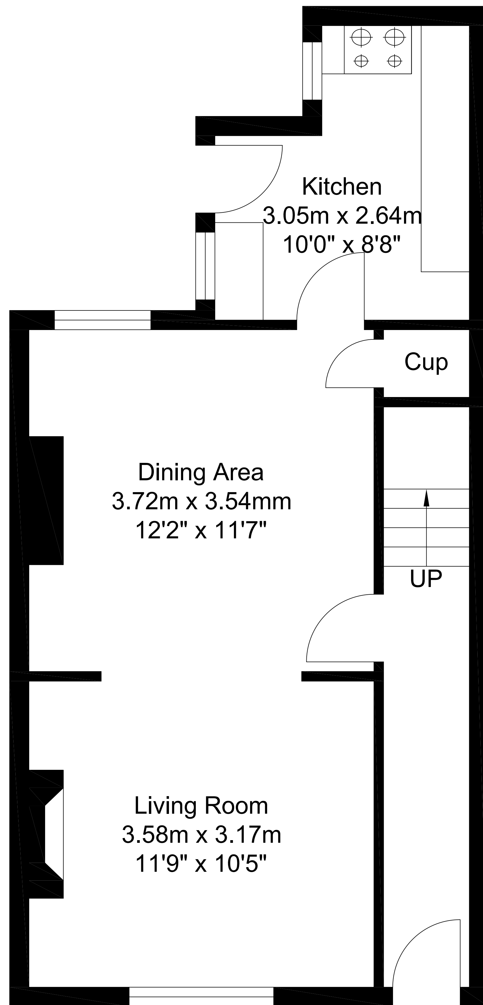
Ground Floor
