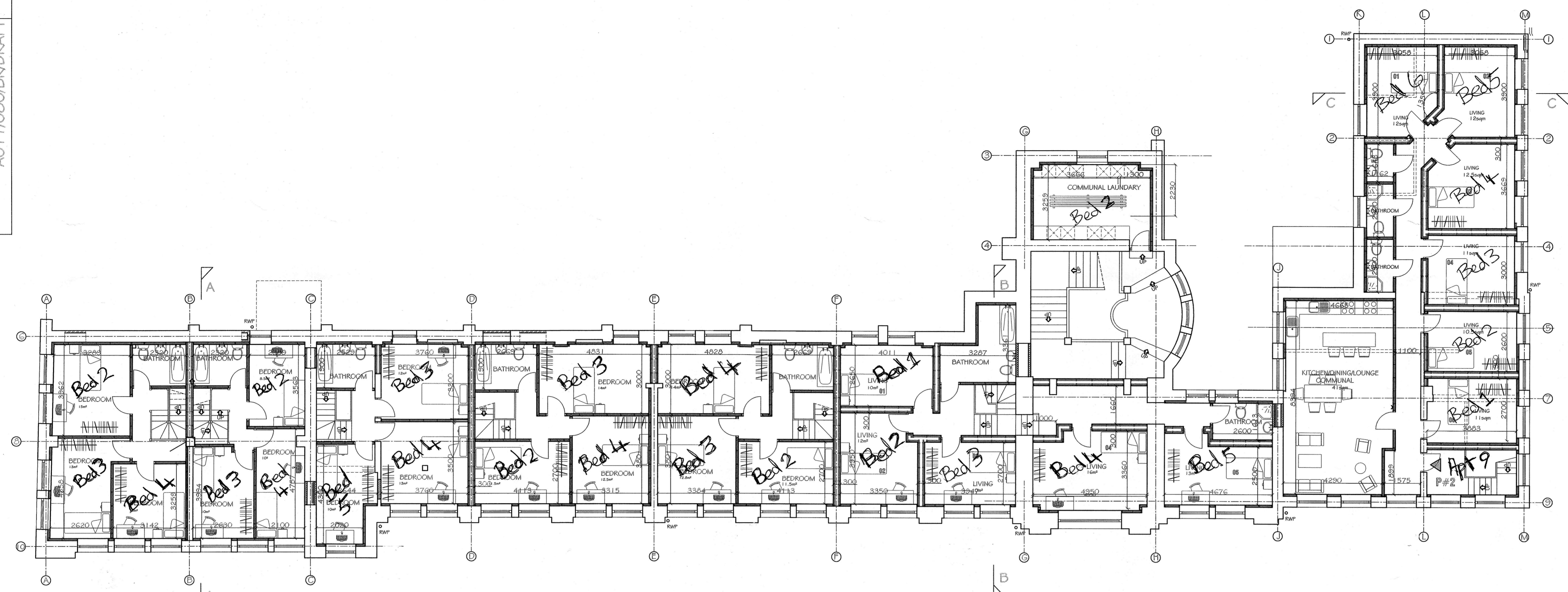
FIRST FLOOR LAYOUT
