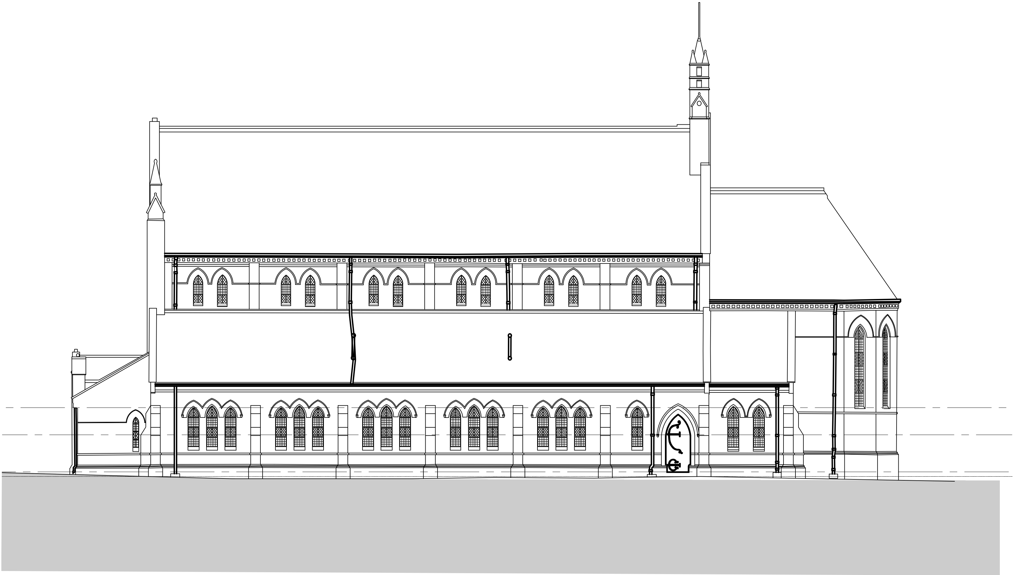
NORTH ELEVATION
