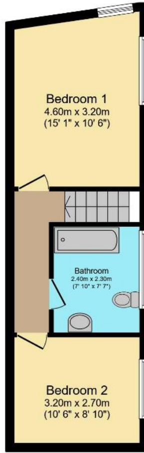
First Floor
