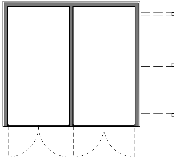
1 202 PLAN - GARAGE PROPOSED SCALE:- 1:100
