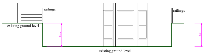
EXISTING WELL ELEVATION SECTION B-B
