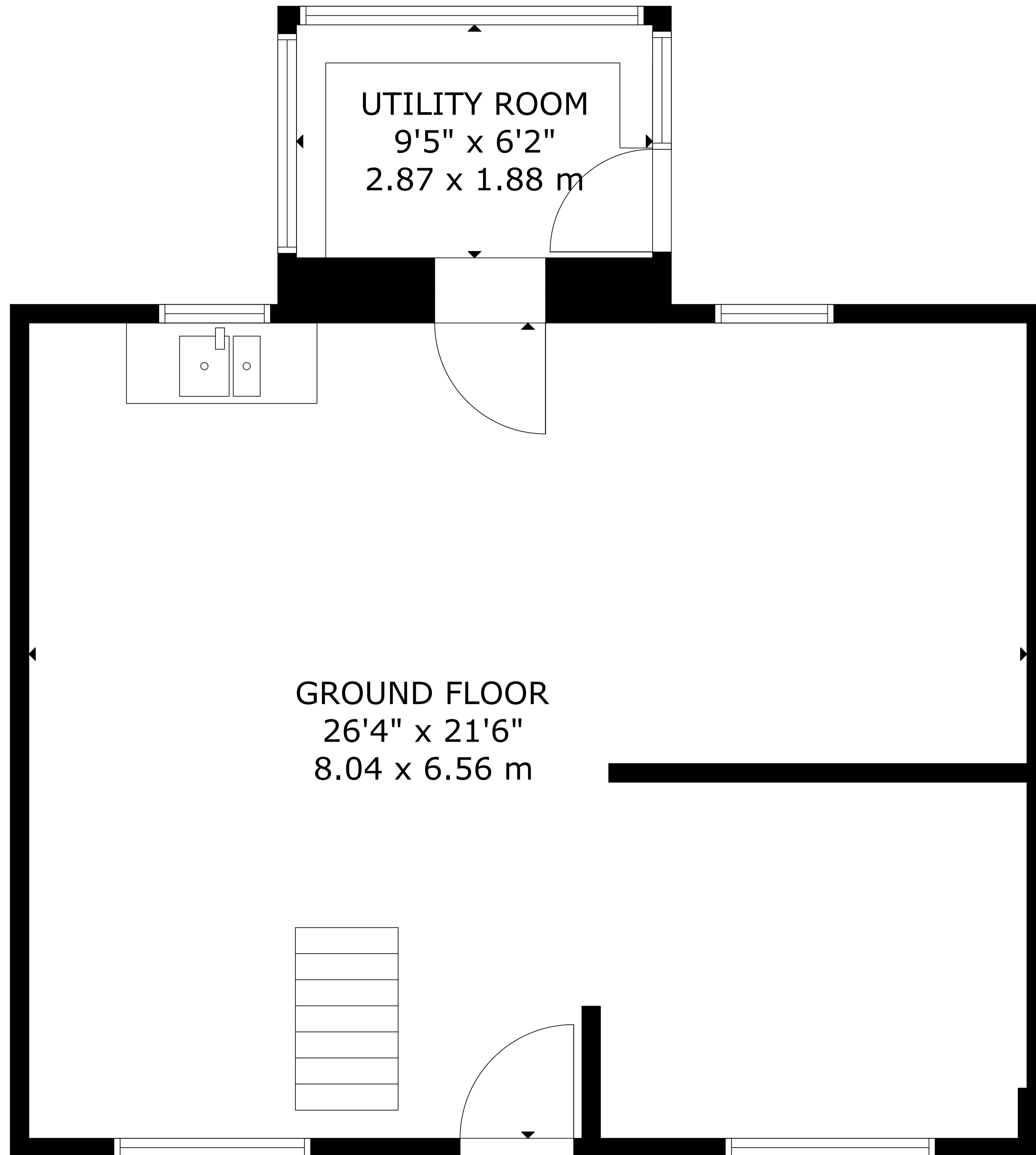
FLOOR 1
