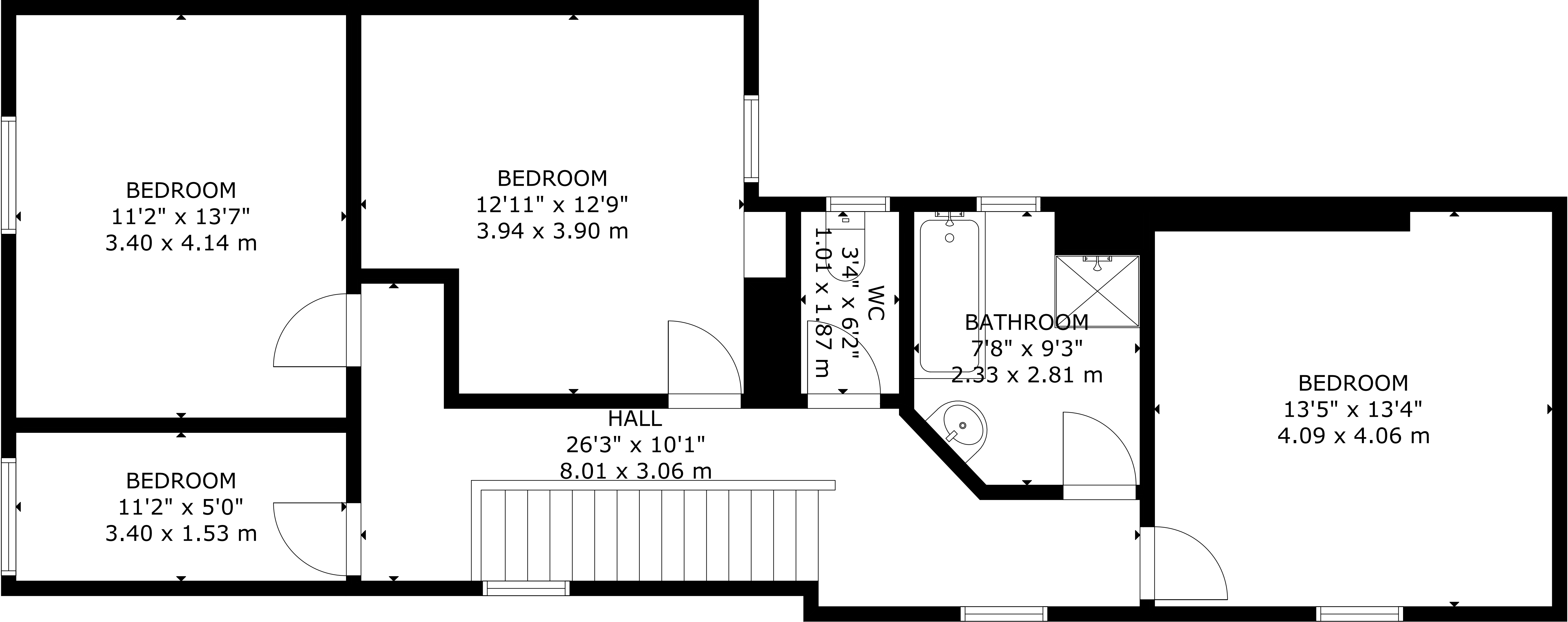
FLOOR 3
