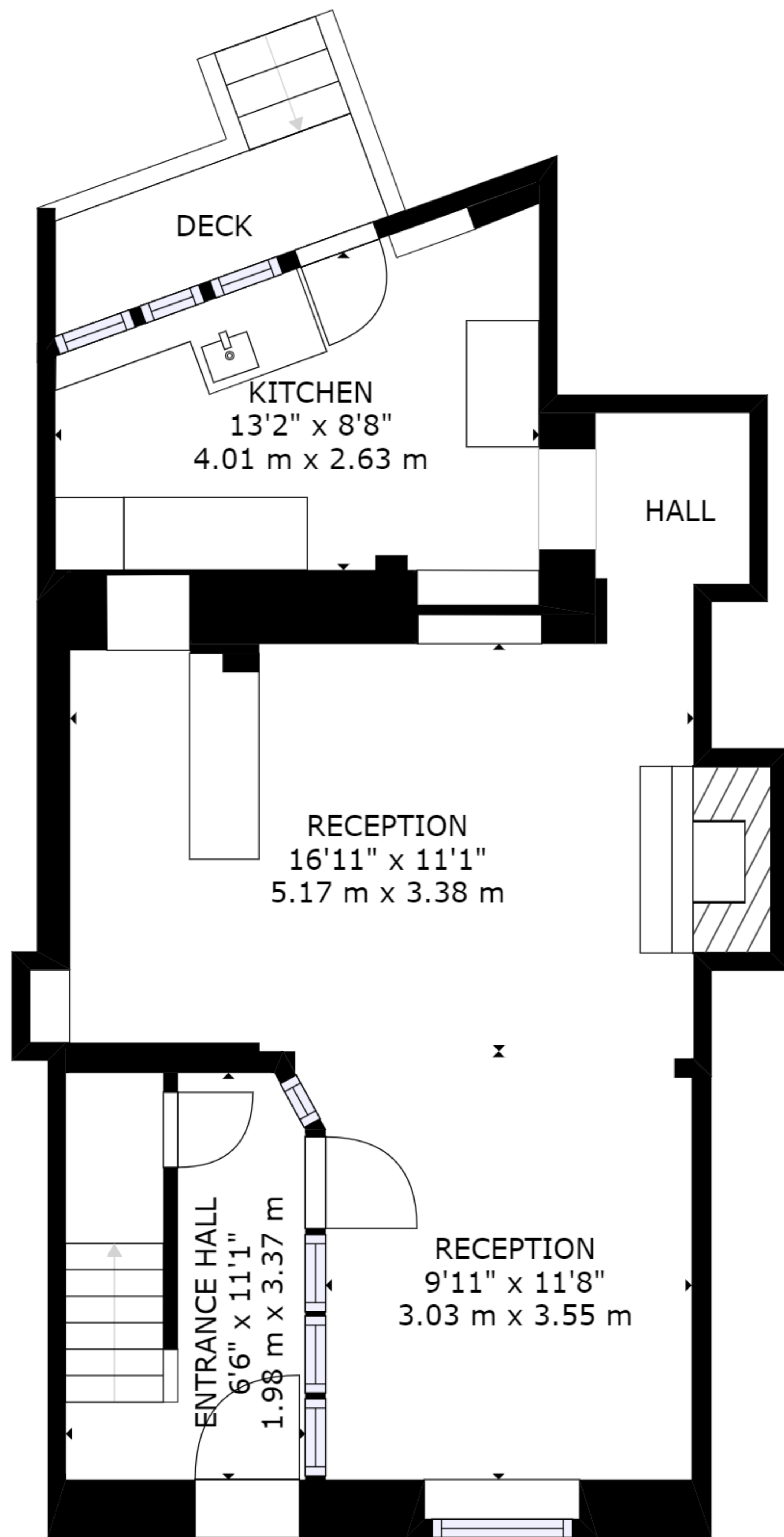
FLOOR 1
