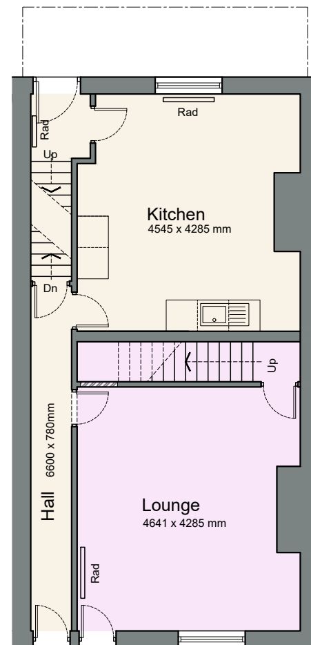
Ground Floor 1:100 @ A3
