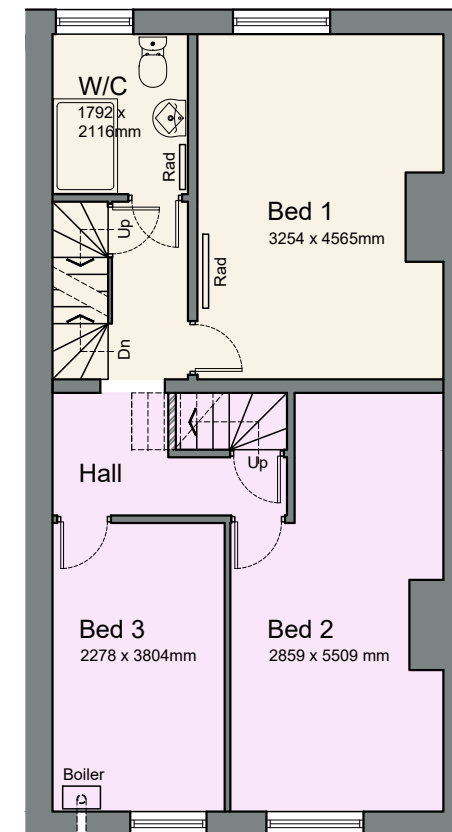
First Floor 1:100 @ A3
