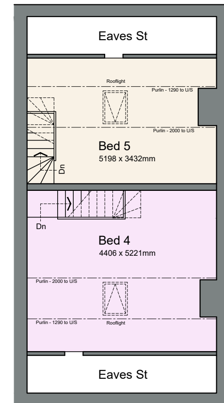
Second Floor/ Roof 1:100 @ A3
