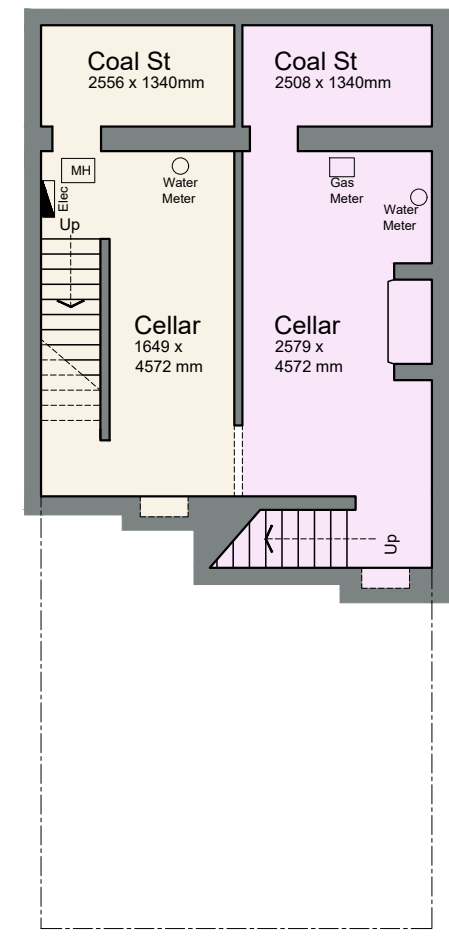
Basement/ Cellar 1:100 @ A3
