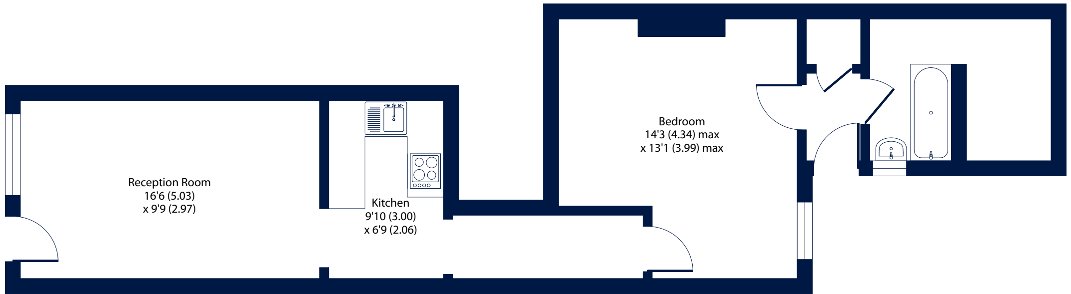
GROUND FLOOR
