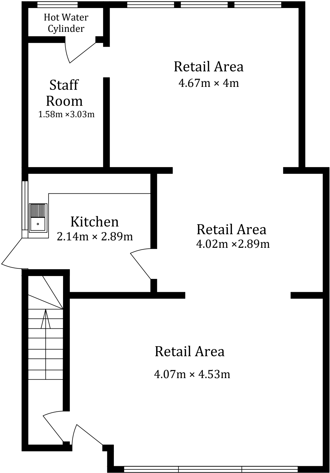
Ground Floor
