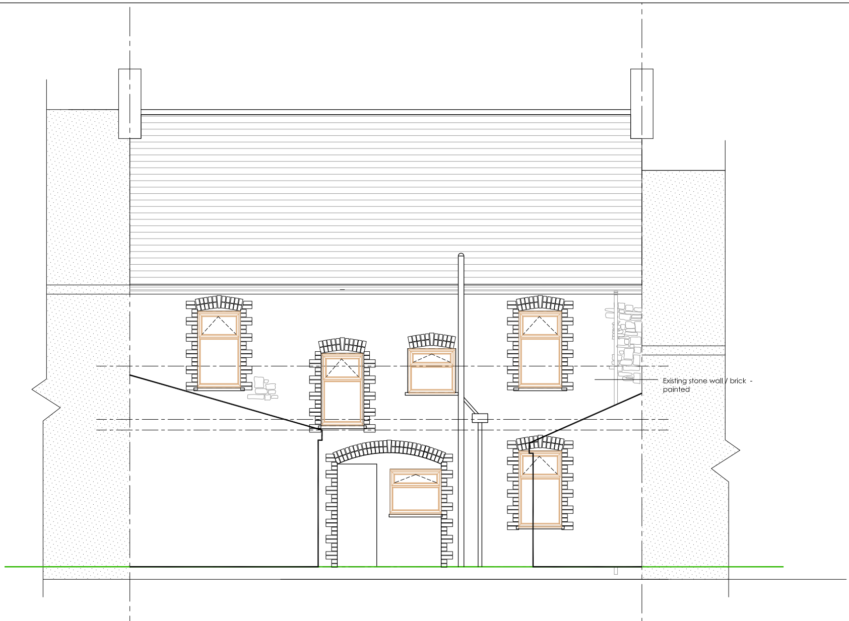
01 EXISTING FRONT ELEVATION SCALE: 1:75
