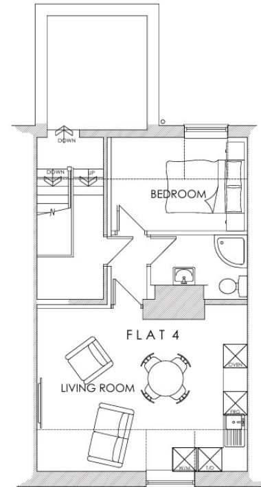
SECOND FLOOR PLAN AS PROPOSED FLAT 4
