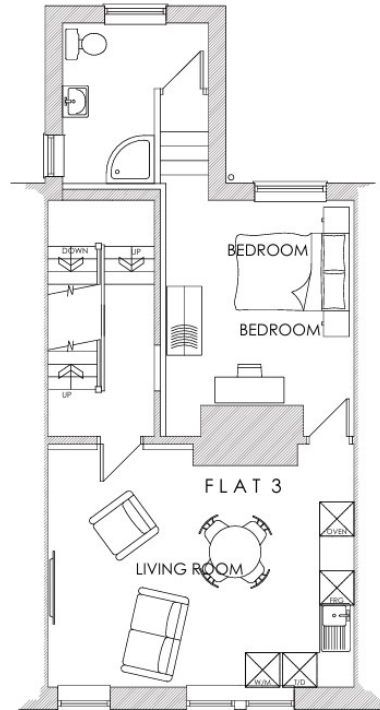
FIRST FLOOR PLAN AS PROPOSED FLAT 3
